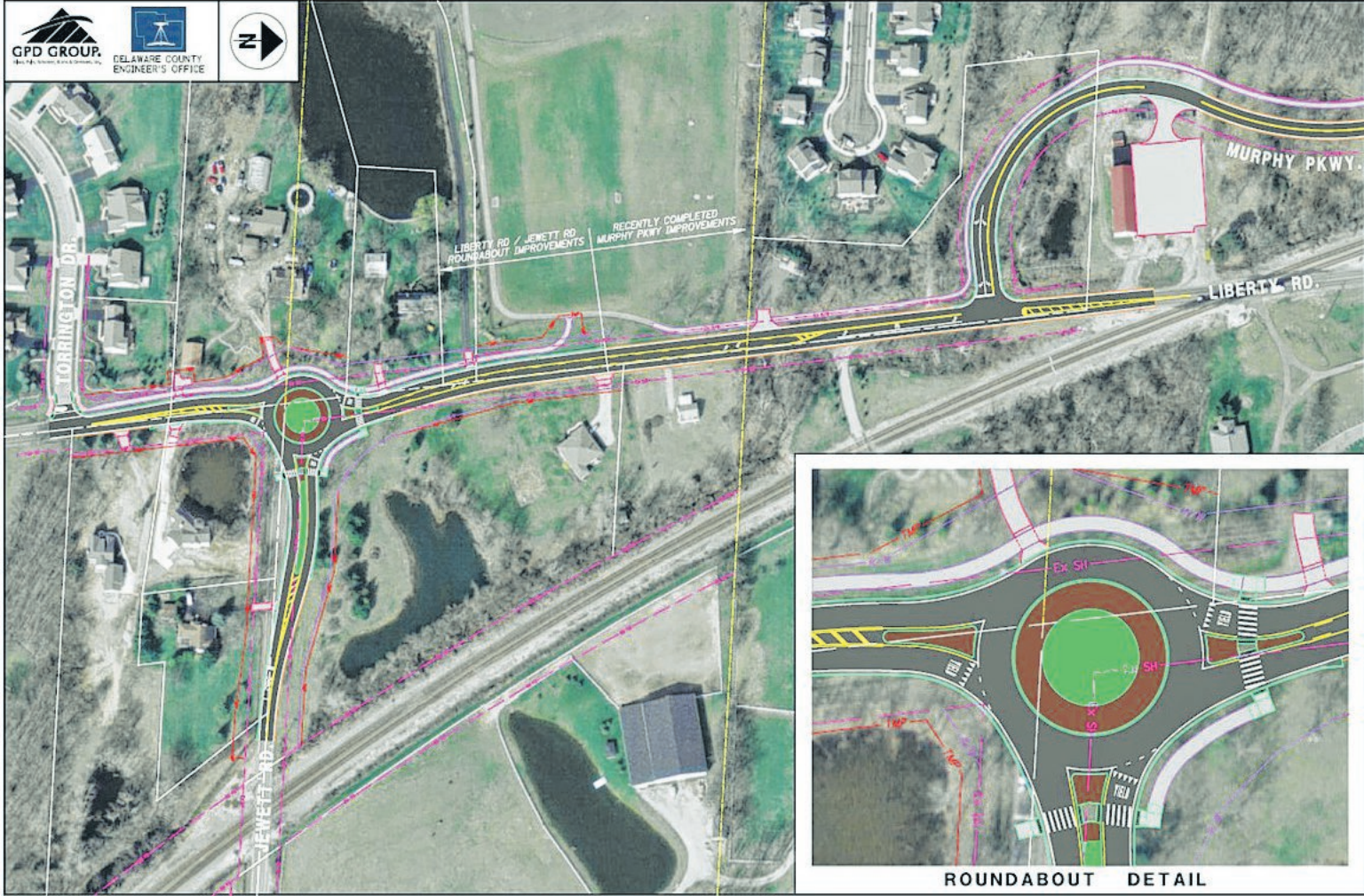
ROUNDABOUT DETAIL
